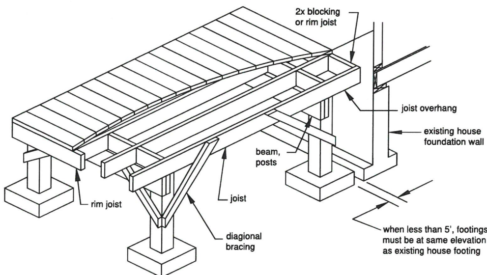
Figure 17 FREE-STANDING DECK
