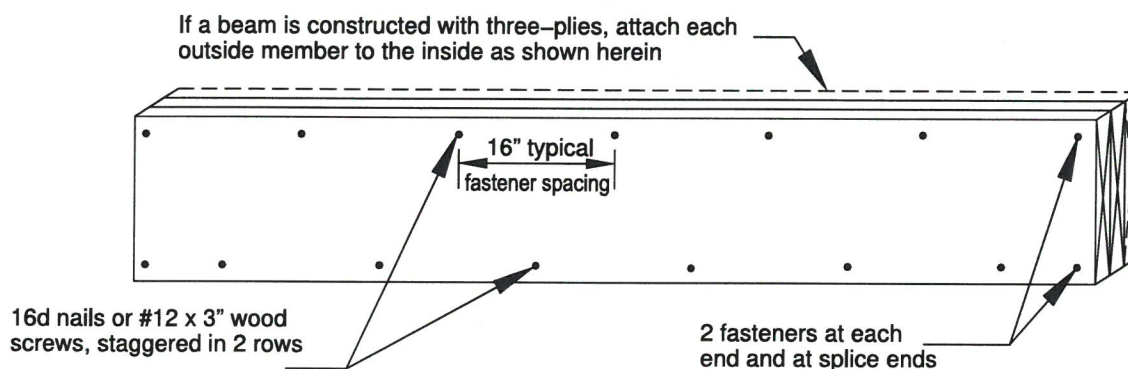
Figure 4 BEAM ASSEMBLY
