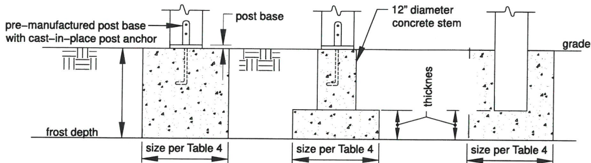
Figure 1 FOOTINGS
