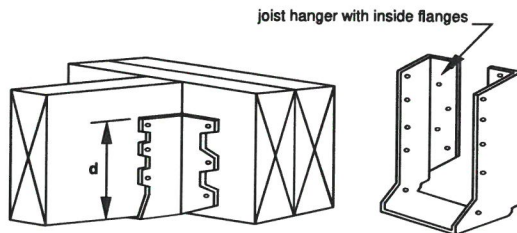
Figure 9 JOIST HANGERS
