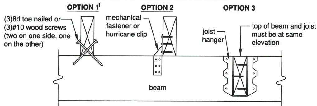
Figure 8 JOIST-TO-BEAM CONNECTIONS
