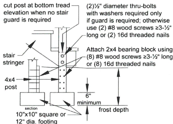
Figure 29 STRINGER BEARING
