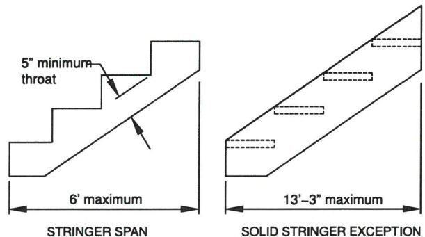
Figure 30 STRINGER SPAN LENGTH
