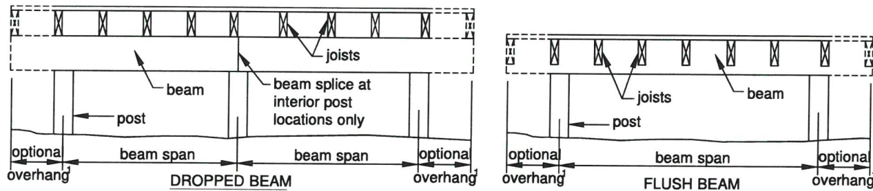
Figure 3 BEAM TYPES
